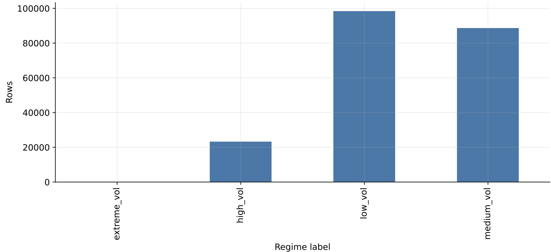
Regime label counts - BTCUSDT 15m HMM
